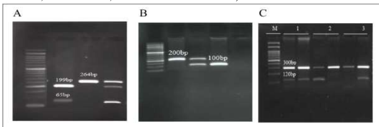
Fig. 1. The gel electrophoresis of genotyped FMO3 variants. A: the different genotypes of rs2266782G/A, lane1: homozygote GG, lane2: heterozygote AG, lane3: homozygote AA; B: the observed genotypes of rs2266780A/G, lane1: homozygote AA, lane2: heterozygote AG, lane3: homozygote GG; C: the genotypes of rs1736557G/A, 1: heterozygote AG, 2: homozygote AA, 3: homozygote GG. M: DNA marker.
